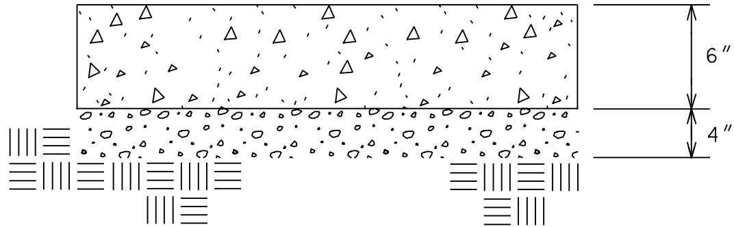
6" PORTLAND CEMENT CONCRETE ON 4" CA-6 CRUSHED GRAVEL
